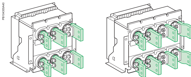
Vertical with spreaders (1250 & 1600A)
