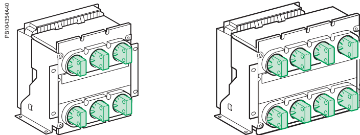
Vertical(800 & 1000A)
